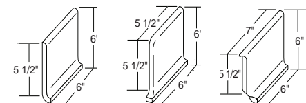
Q3565 Cove Base Q3565 L/R Cove Base Outside Corner Q3565B Cove Base Inside Corner
